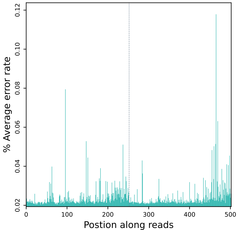
Error rate distribution along reads (R10421)
